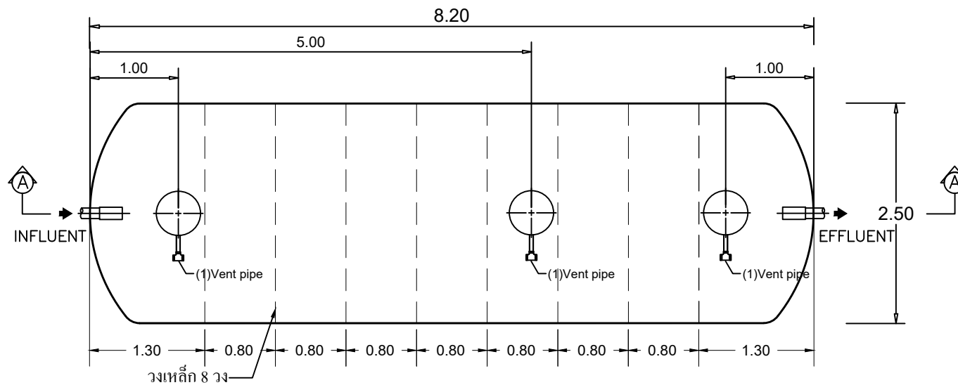
STAR TANK MODEL PT-40FB
