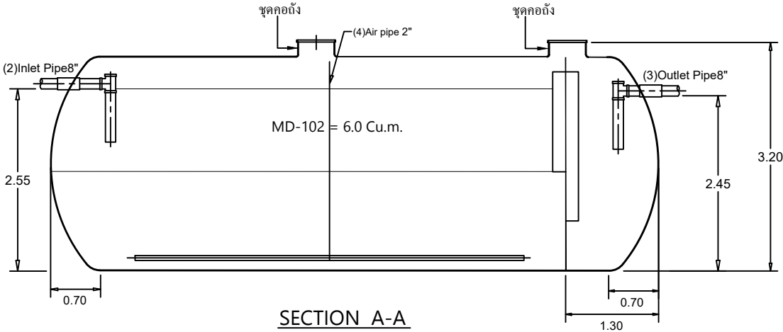
STAR TANK MODEL CFRBST-60Q
