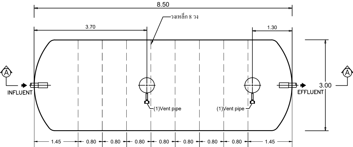
STAR TANK MODEL CFRBST-60Q
