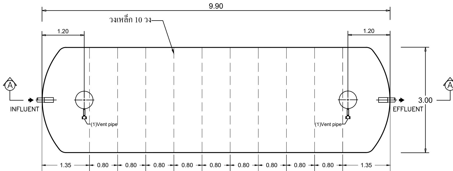
STAR TANK MODEL CFRBCF-70Q
