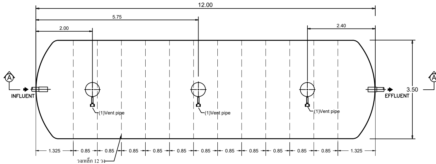
STAR TANK MODEL CFRBSS-115Q
