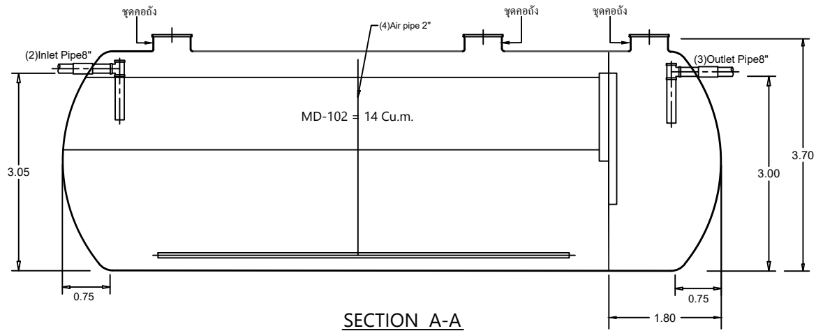
STAR TANK MODEL CFRBST-100Q
