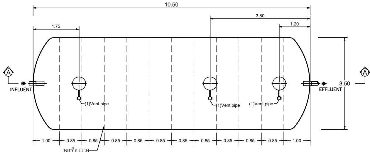
STAR TANK MODEL CFRBST-100Q
