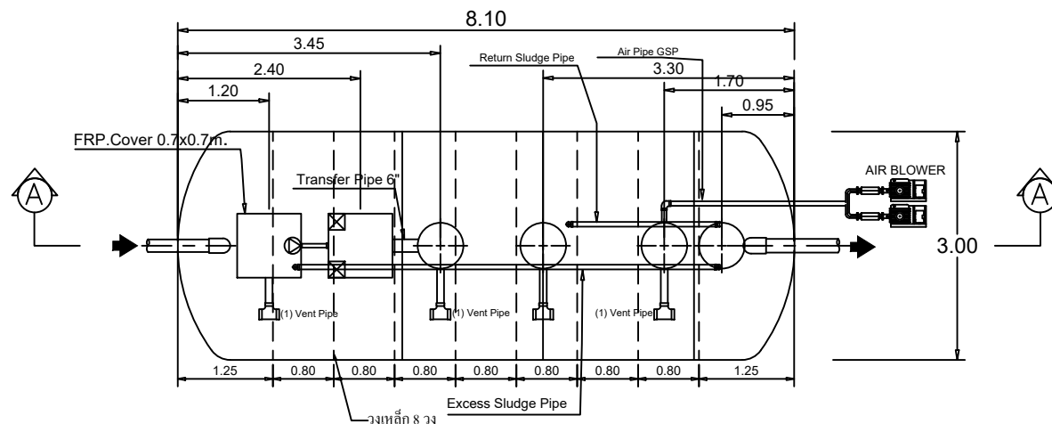
STAR SSA-18800D3 PLAN VIEW
