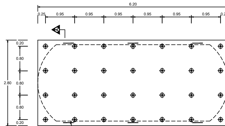
BOTTOM PLAN
