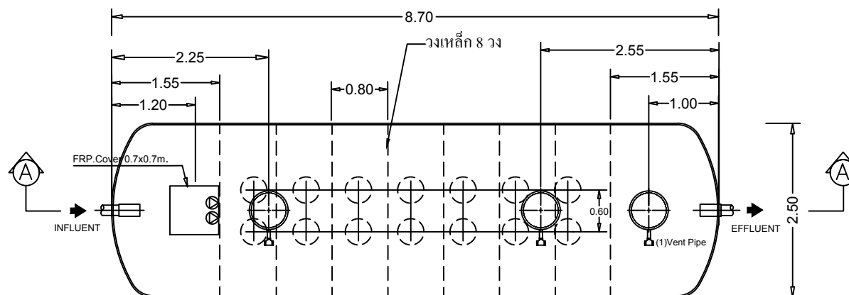
STAR TANK MODEL SSA-2537ZR
