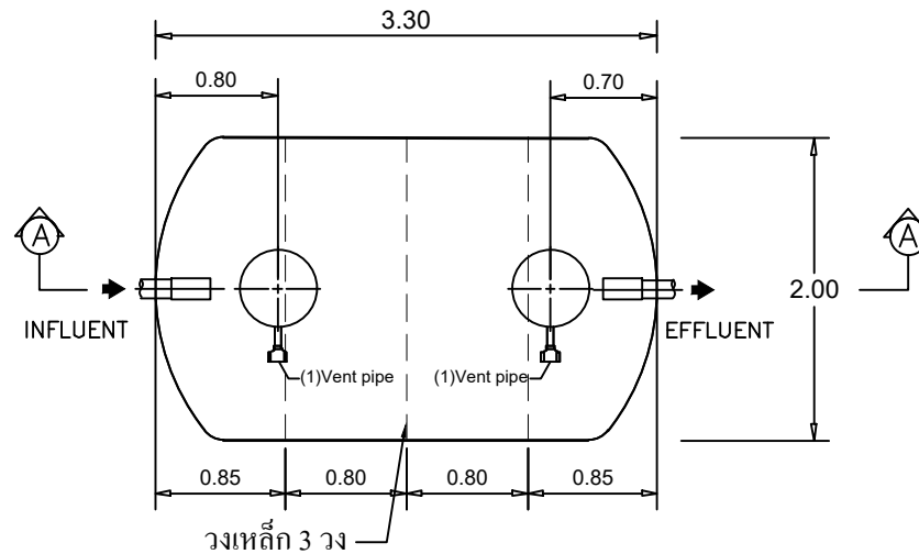
STAR TANK MODEL HFF-40A
