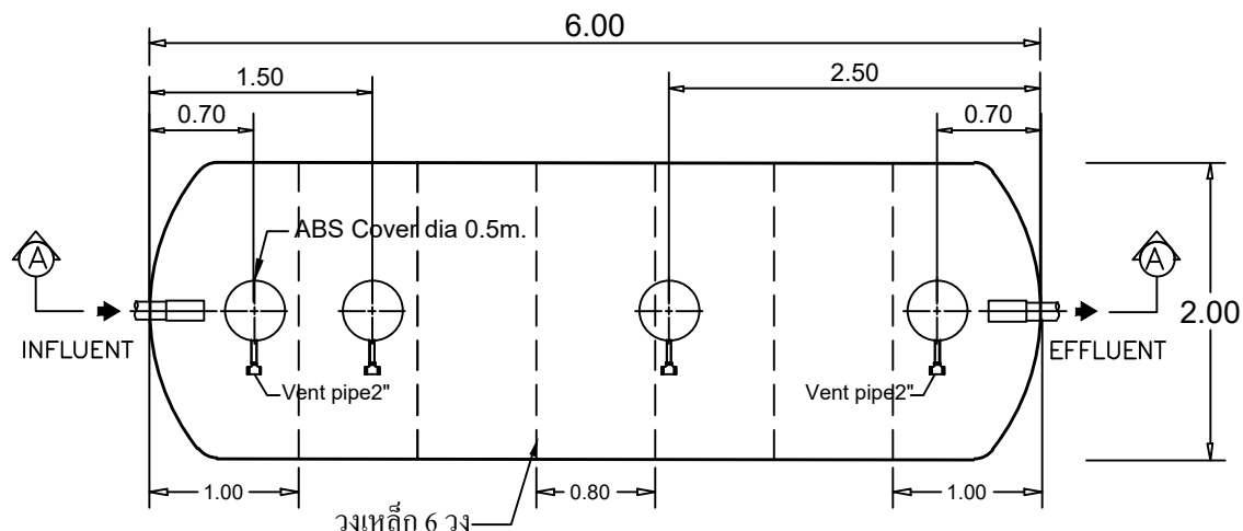
STAR TANK MODEL PSP-F6-A
