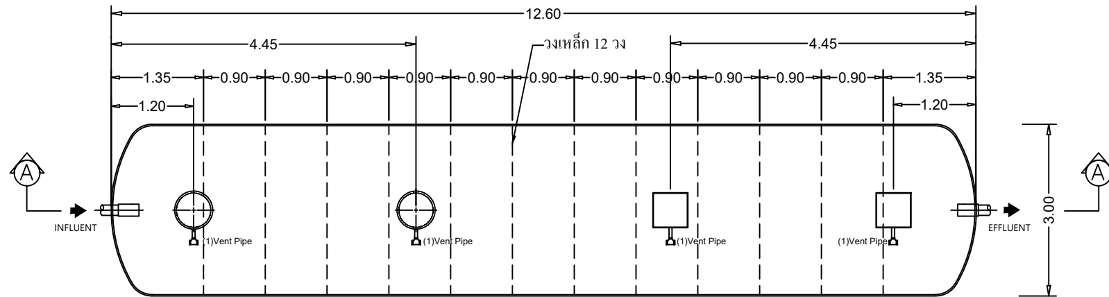
STAR TANK MODEL WSA-3085Z
