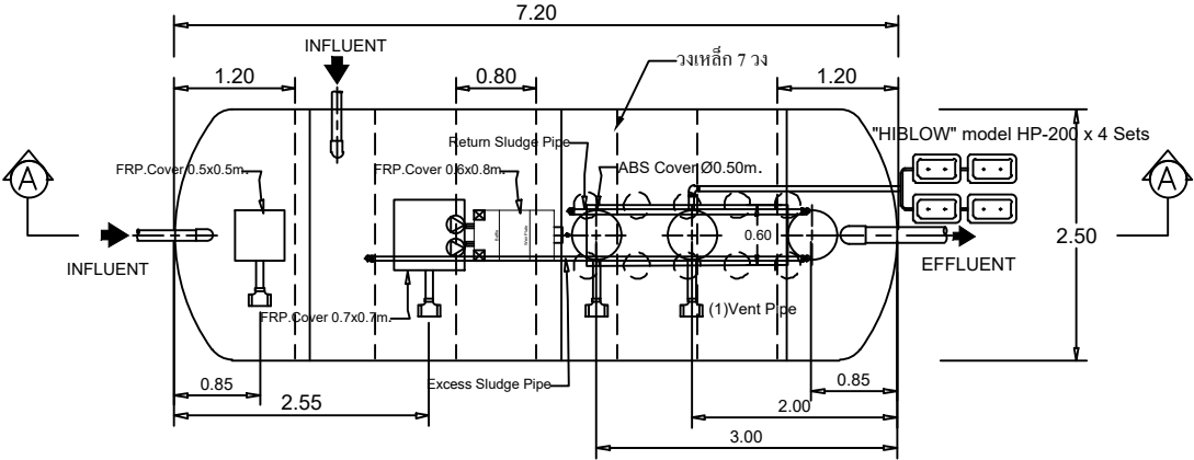
STAR SK-14600Z PLAN VIEW
