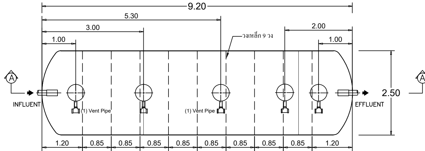
STAR TANK MODEL C-25050-B
