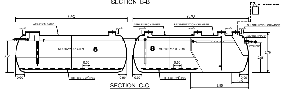
SECTION C-C
