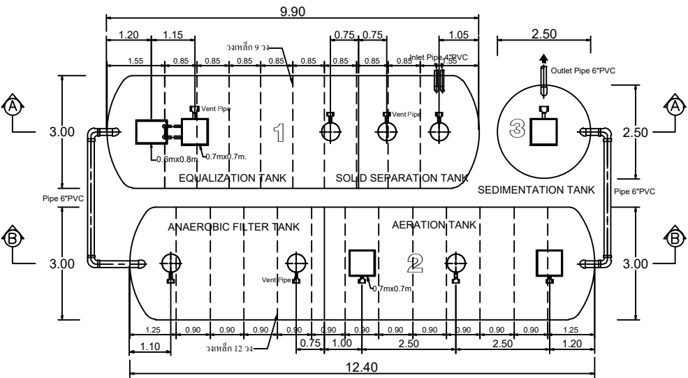
STAR SA-65800E PLAN VIEW
