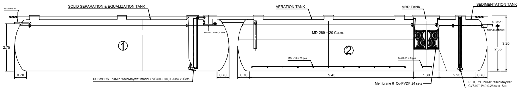
SECTION A-A SCALE NTS
