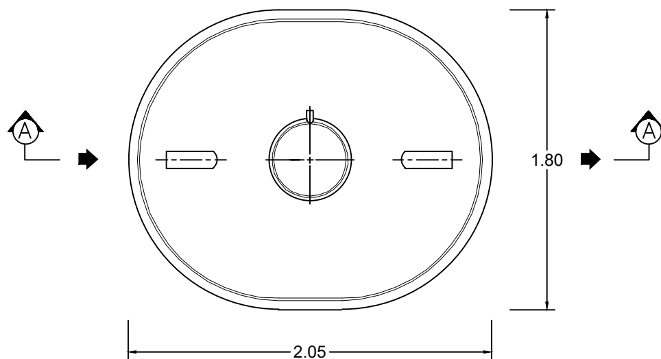
PLAN VIEW
