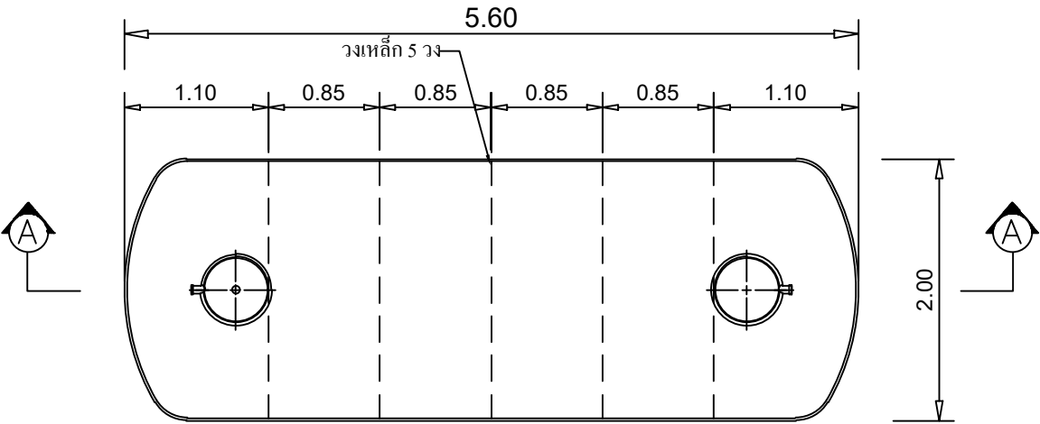
STAR TANK MODEL SW-2015
