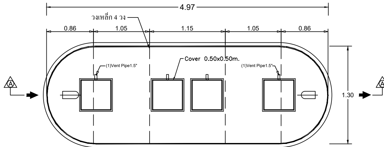
PLAN VIEW
