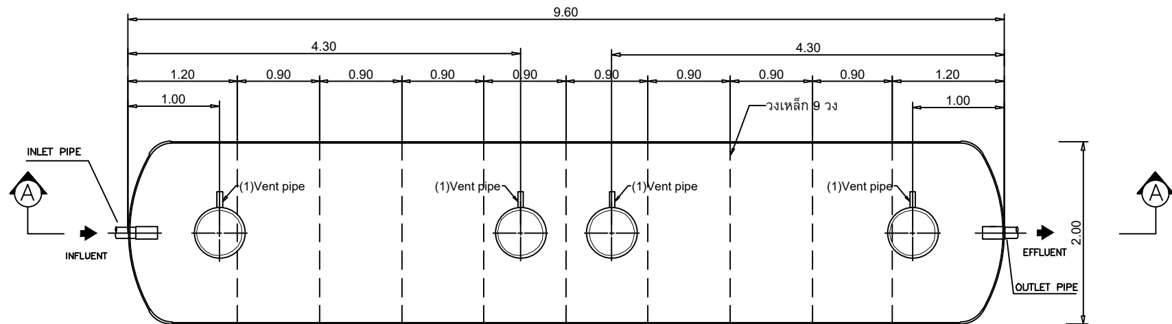
STAR TANK MODEL SS-2026K
