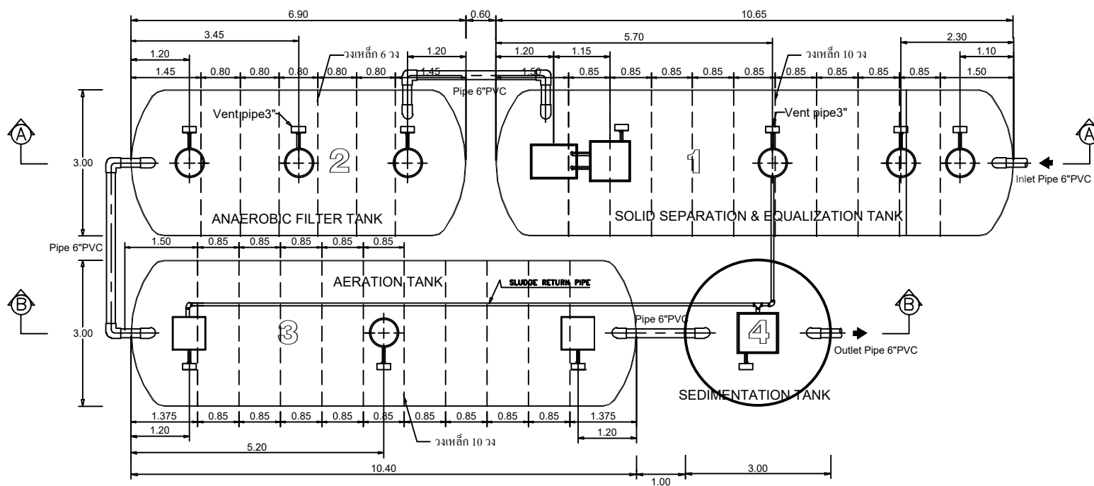
SA-80800E (ONGROUND) PLAN VIEW
