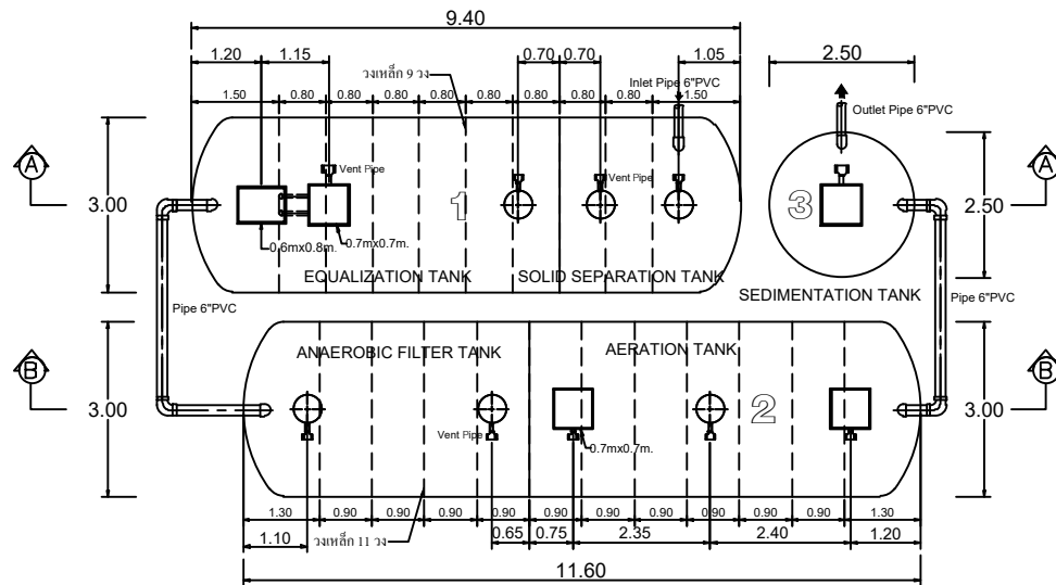
STAR SA-60800E PLAN VIEW
