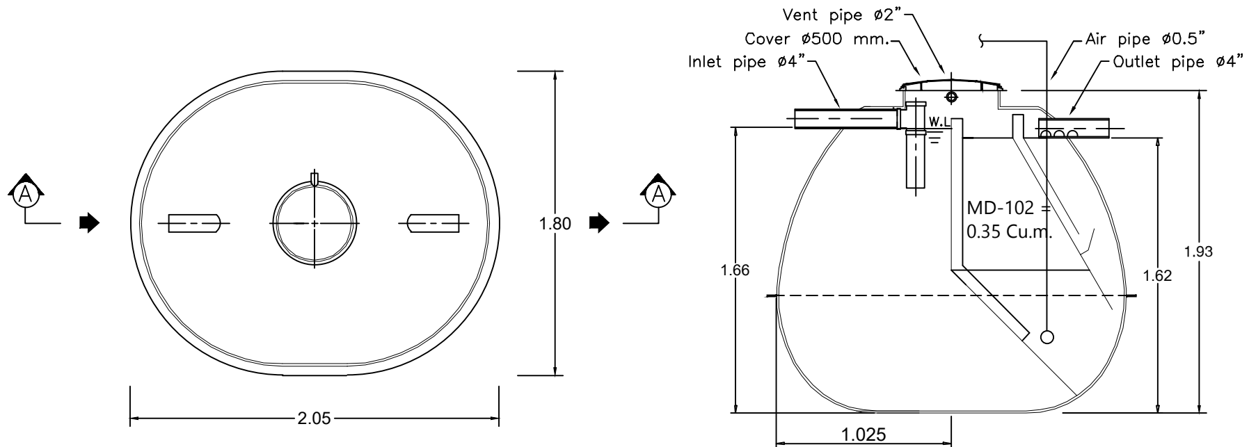
PLAN VIEW
